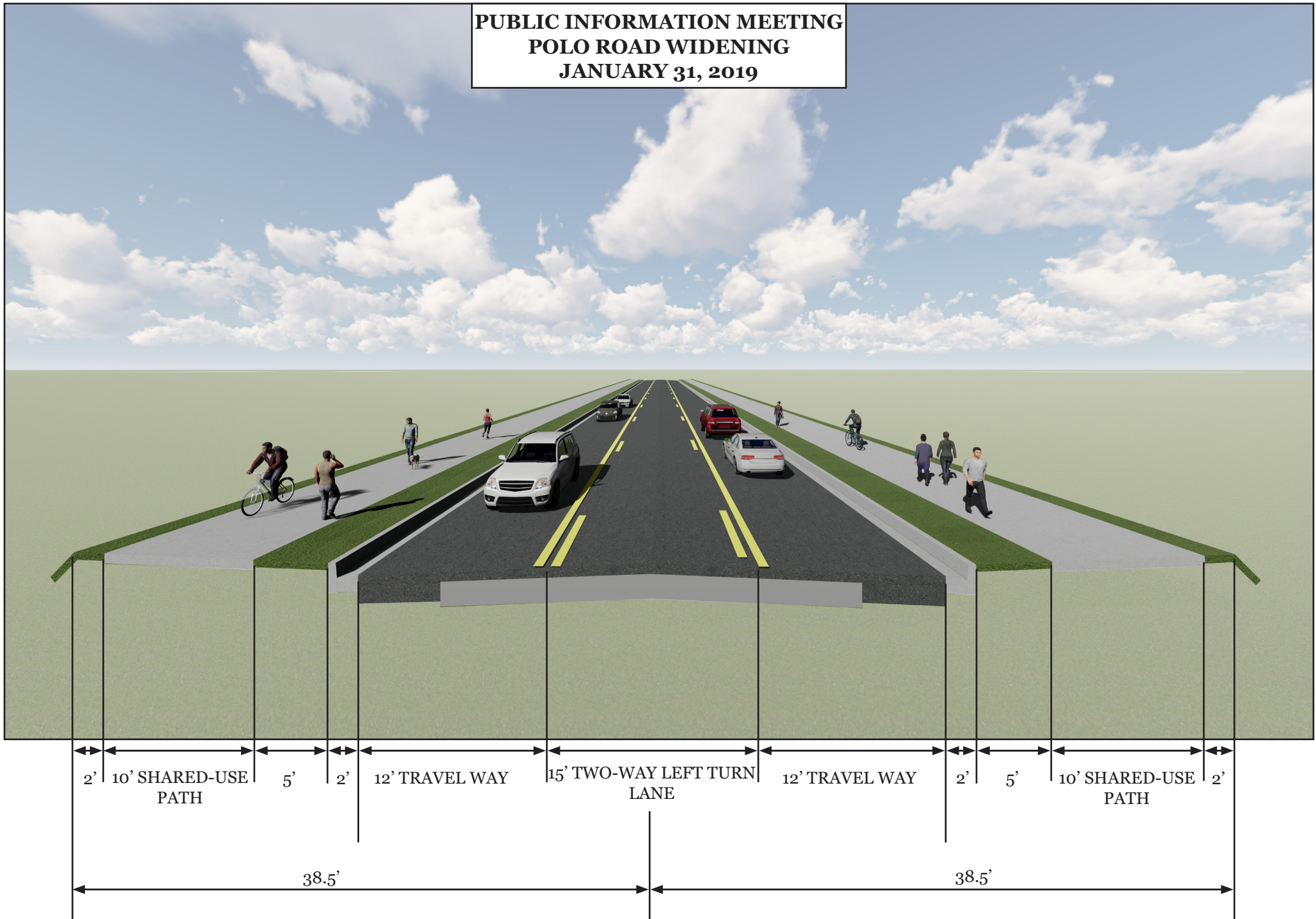
TYPICAL SECTION B
